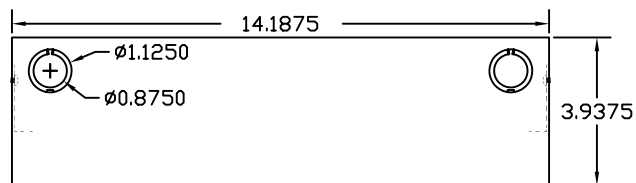
BACKBOX TOP/BOTTOM VIEW
